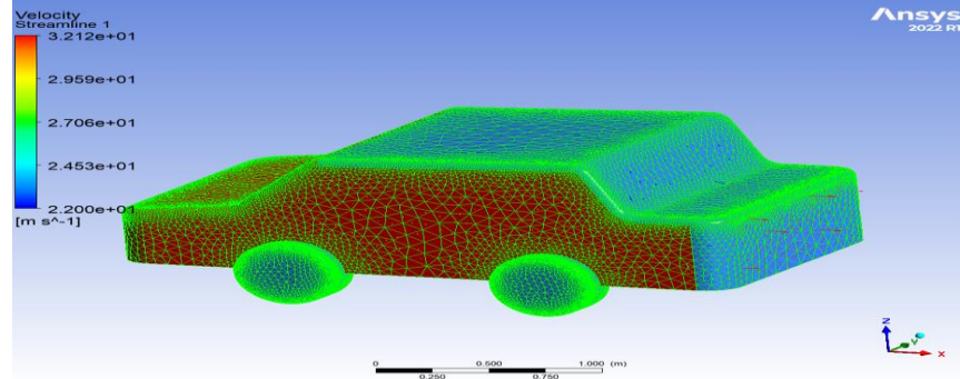
Figure 16: Velocity streamline at 30 m/sec
