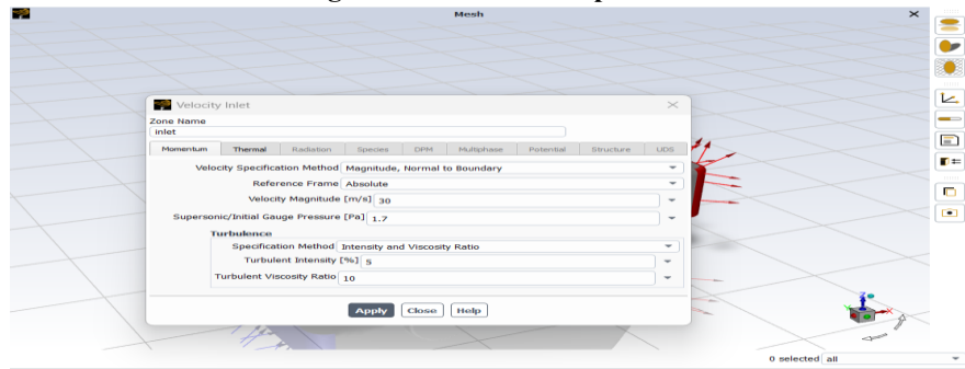
Figure 14: Inlet boundary conditions
