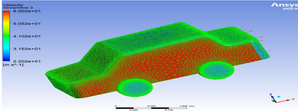
Figure 22: Velocity Stream line at 60 m/sec
