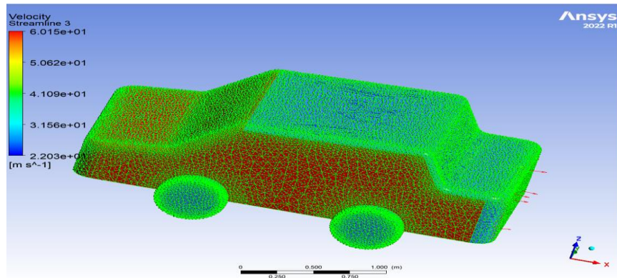
Figure 18: Velocity Stream line at 60 m/sec
