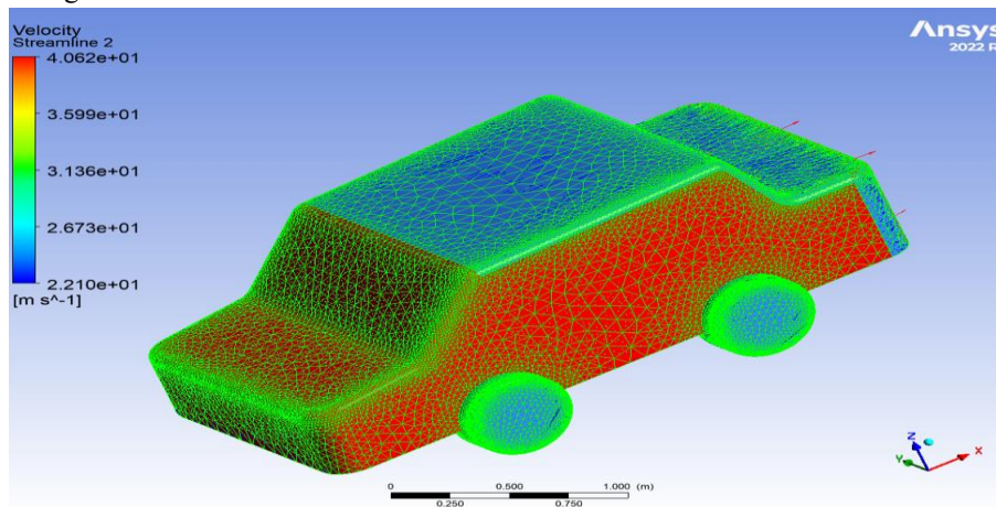
Figure 21: Velocity Stream line at 40 m/sec
