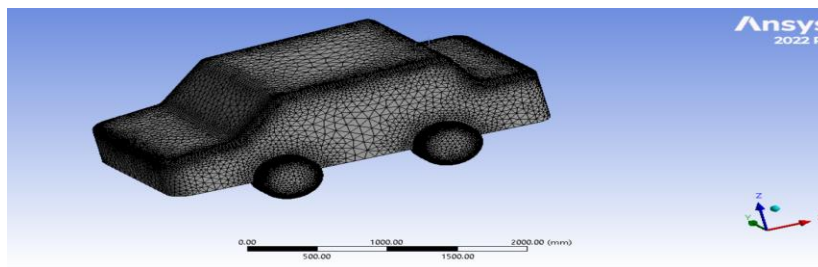
Figure 8: Meshing model
