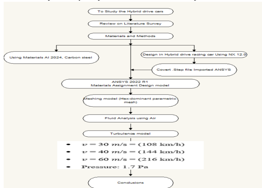
Figure 2: Design flow chart
