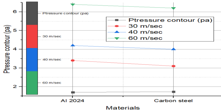
Figure 23: Air flow analysis using hybrid Car with different Materials maximum flow velocity conditions at pressure 1.7 pa
