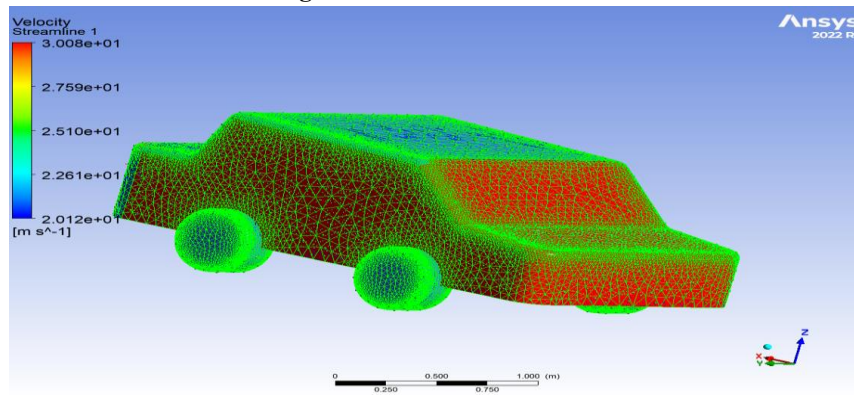
Figure 20: Velocity Stream line at 30 m/sec
