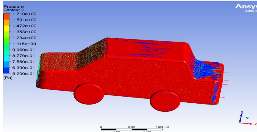
Figure 19: Pressure Contour
