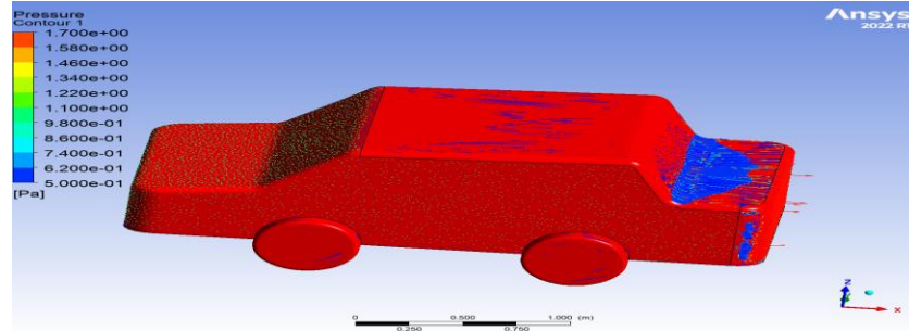
Figure 15: Pressure Contour
