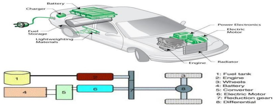
Figure 1: hybrid drive car schematic view
