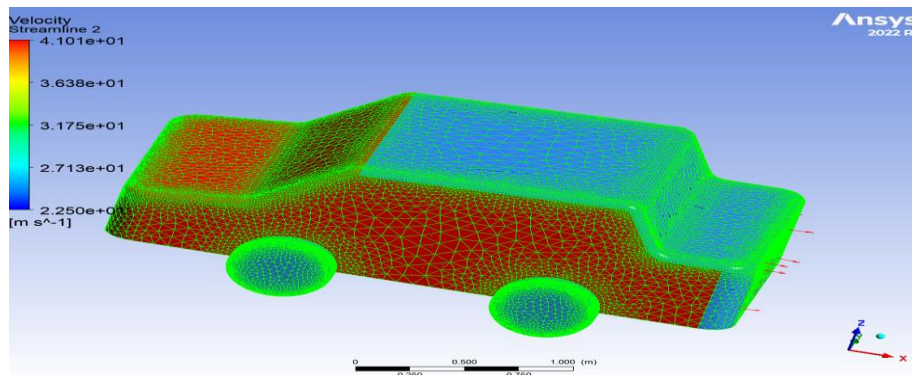
Figure 17: Velocity Stream line at 40 m/sec
