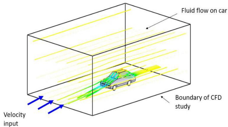
Figure 5: Boundary Condition of CFD analysis
