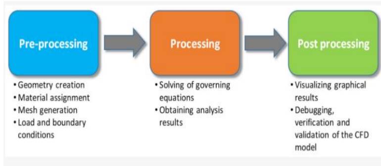
Figure 10: Computational fluid dynamics stages
